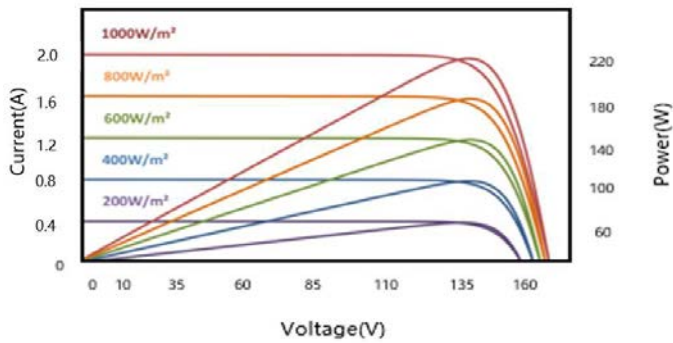
COM-CBS1 at different light intensities
