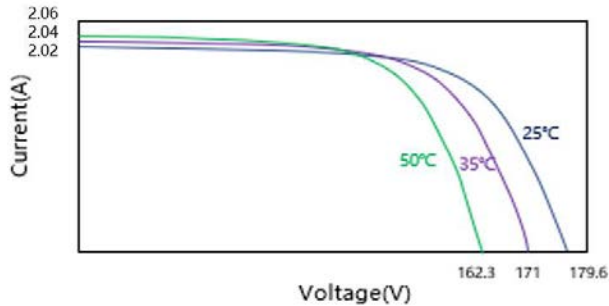
COM-CBS1 at different temperatures
